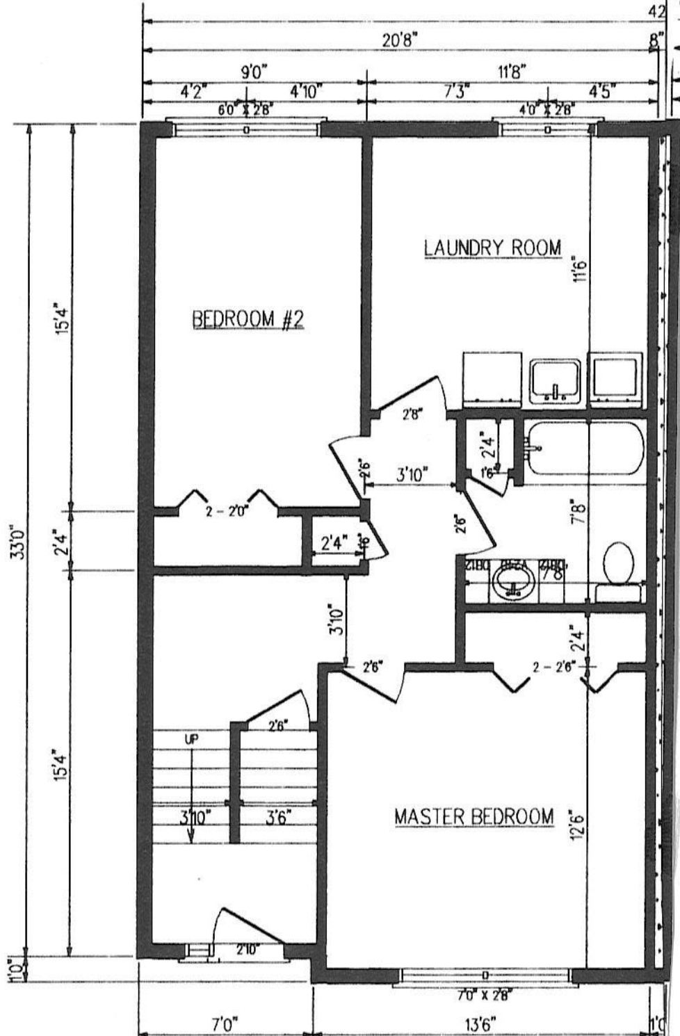
CAMBRIDGE SEMI-DETACHED HOME BASEMENT LEVEL
