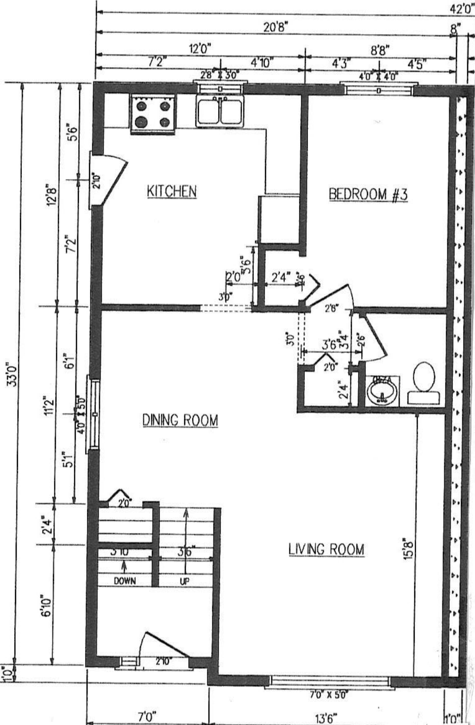
CAMBRIDGE SEMI-DETACHED HOME MAIN FLOOR LEVEL
